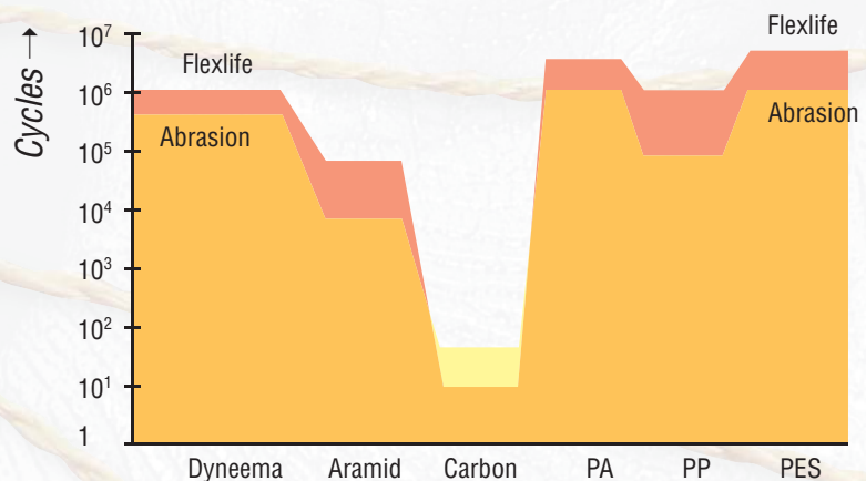
Abrasion resistance and flexlife
